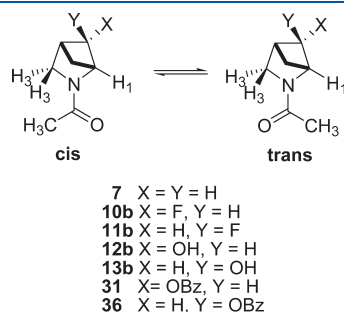
Figure 2. Amide conformations for methanopyrrolidines.
